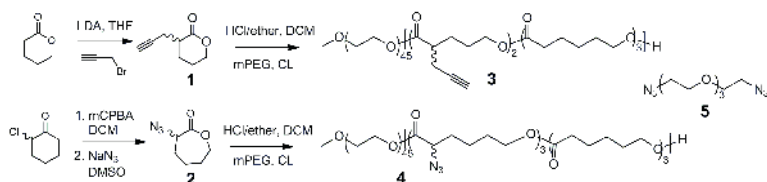
Fig. 1: Synthesized monomers ( \alpha -propargyl- \delta -valerolactone 1 , \alpha -azido- \epsilon -caprolactone 2 ) and polymers ( 3 , 4 ); 5 was commercially obtained.
